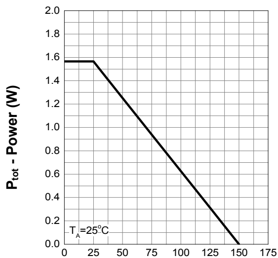
Power Capability
