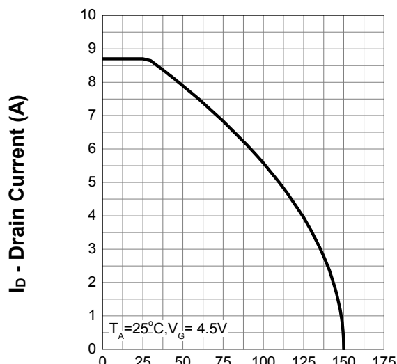
Current Capability
