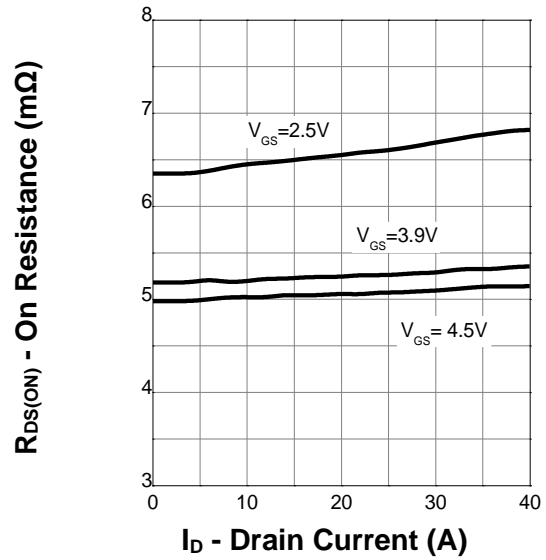
On Resistance
