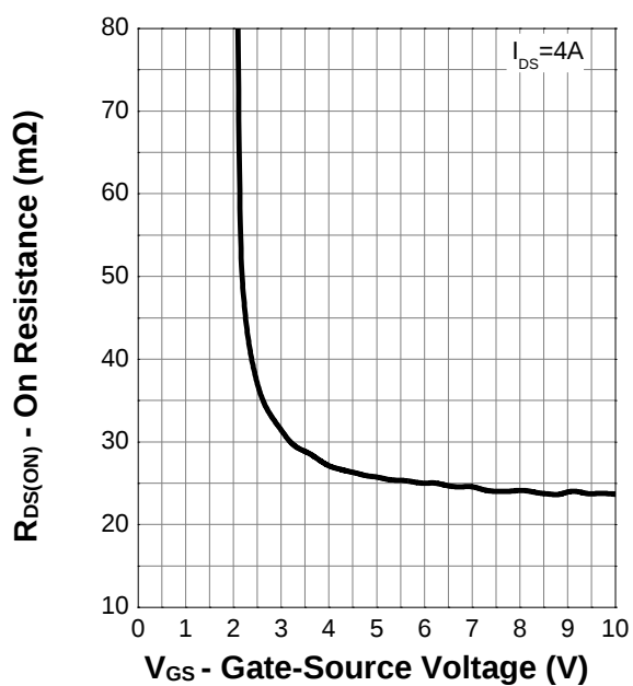
Transfer Characteristics
