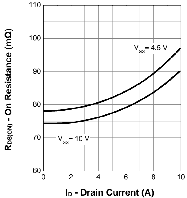
On Resistance
