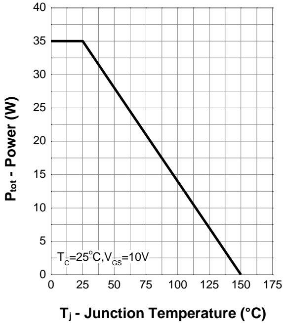
Power Capability
