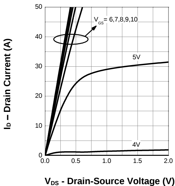
Output Characteristics
