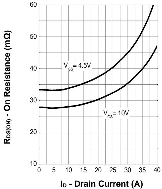
On Resistance
