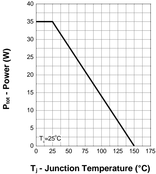
Power Capability
