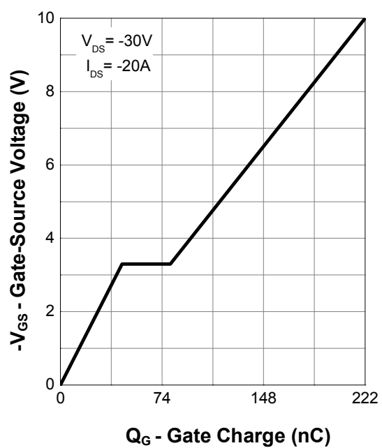
Gate Charge
