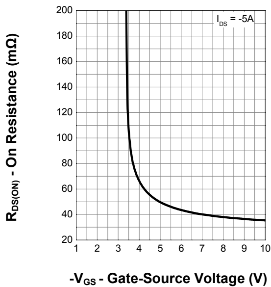
Transfer Characteristics
