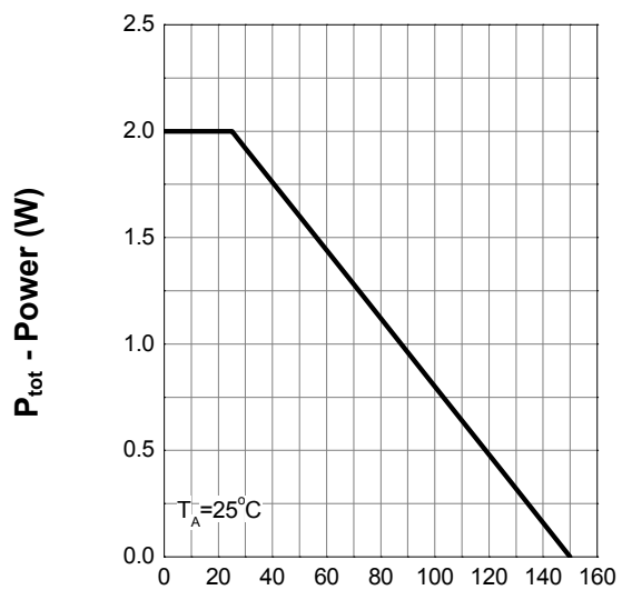
Power Dissipation
