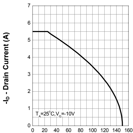
Drain Current
