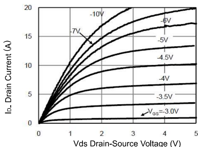
Figure 3 Output Characteristics
