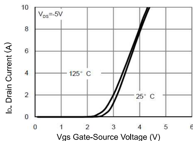
Figure 5 Transfer Characteristics
