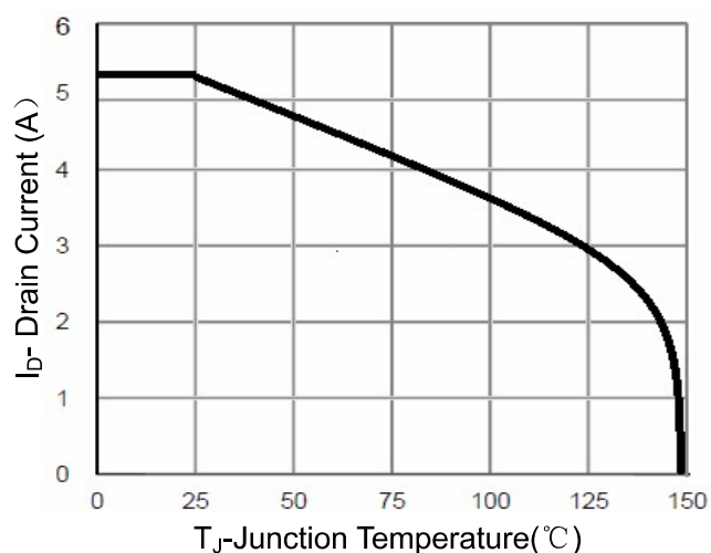
Figure 2 Drain Current
