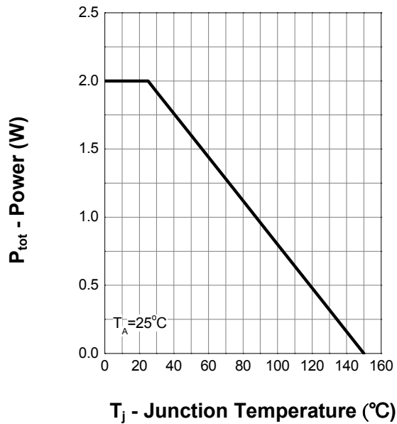
Power Dissipation
