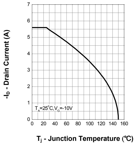
Drain Current
