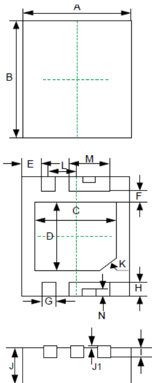
DFN2×3-6L
