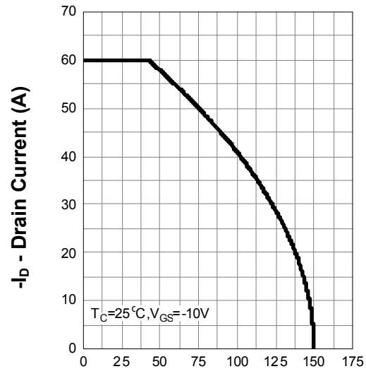
Current Capability
