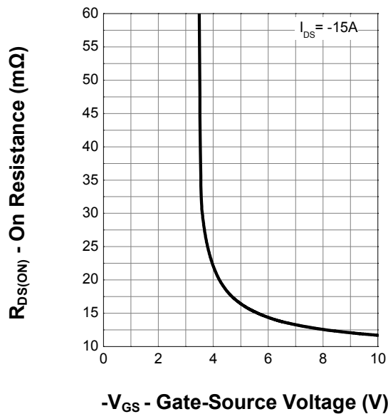
Transfer Characteristics
