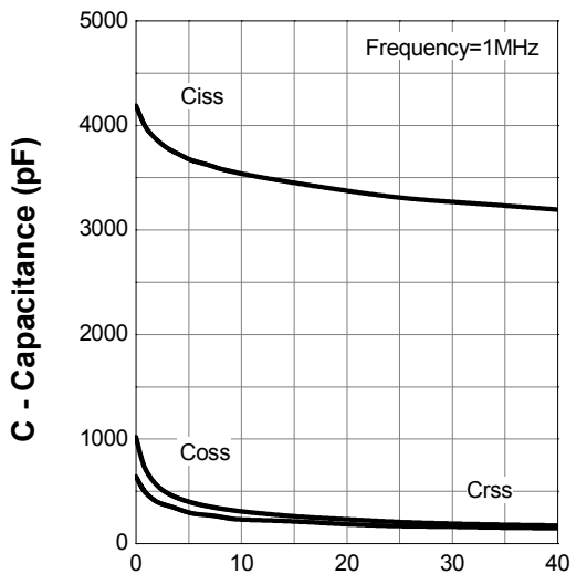
Capacitance
