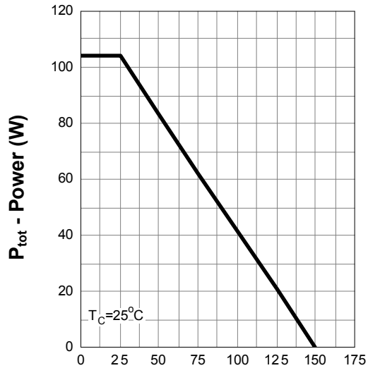
Power Capability
