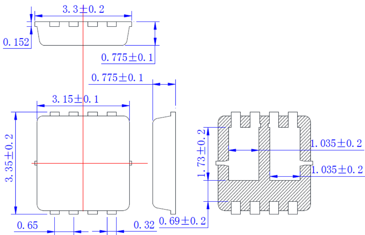
PDFN3.3x3.3-8L Package
