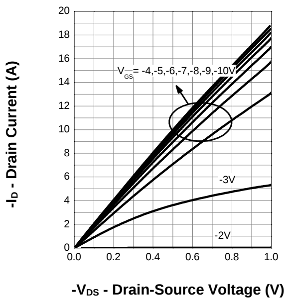
Output Characteristics
