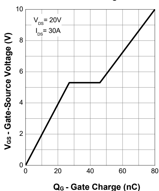
Gate Charge
