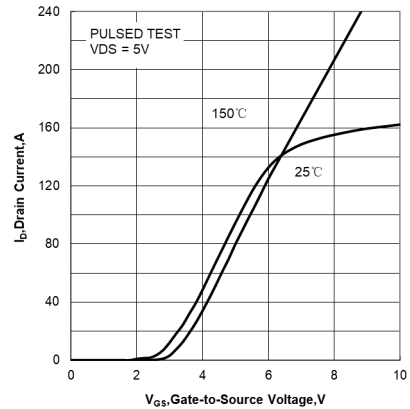
Figure 2. Transfer Characteristics
