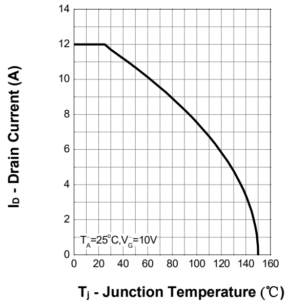
Drain Current
