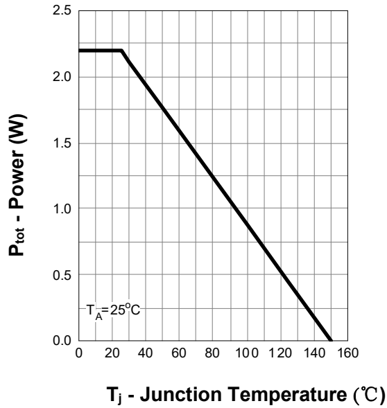
Power Dissipation
