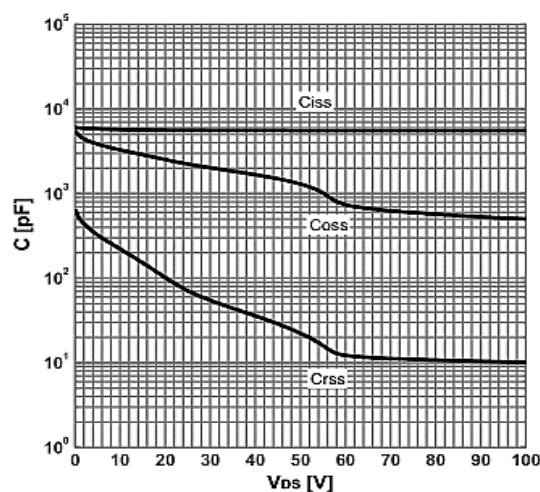
Figure9 Typ. capacitances
