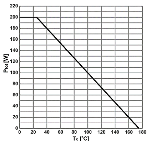
Figure 1. Power dissipation
