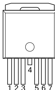
Top View TO-263-7L
