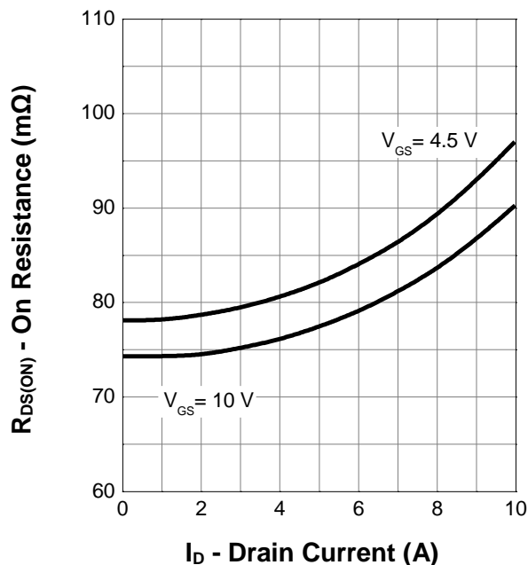
On Resistance
