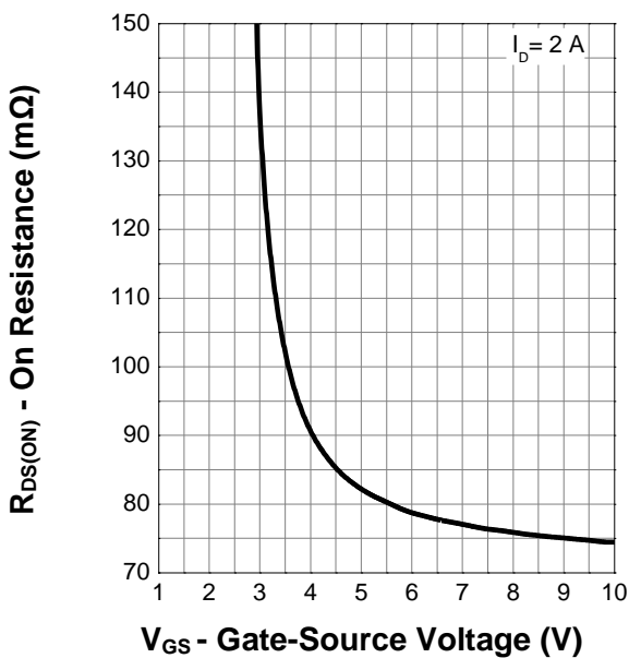
Transfer Characteristics
