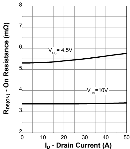
On Resistance
