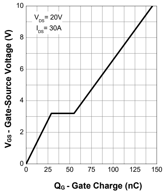
Gate Charge
