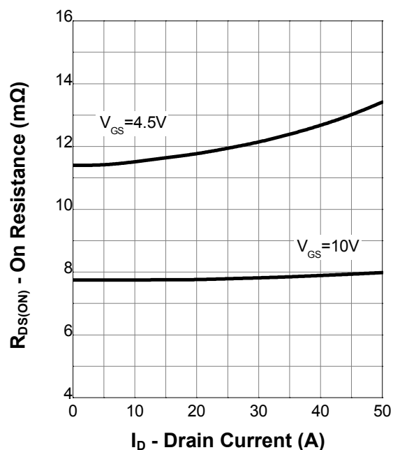
On Resistance
