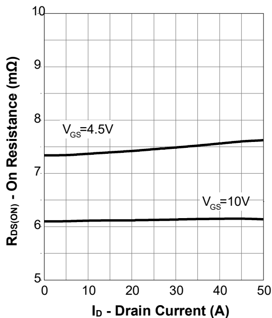
On Resistance
