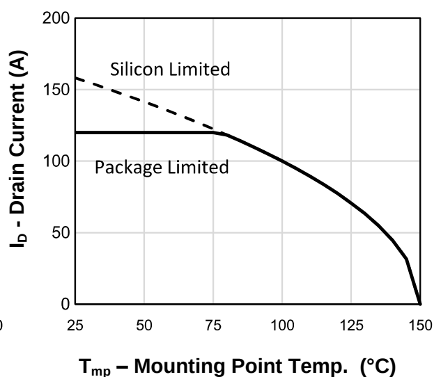
Current Capability
