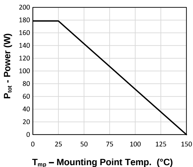
Power Capability
