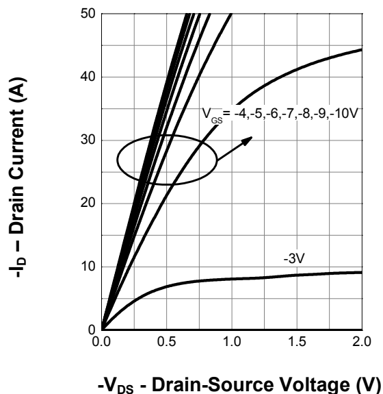
Output Characteristics
