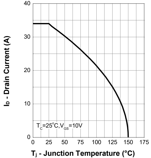
Current Capability
