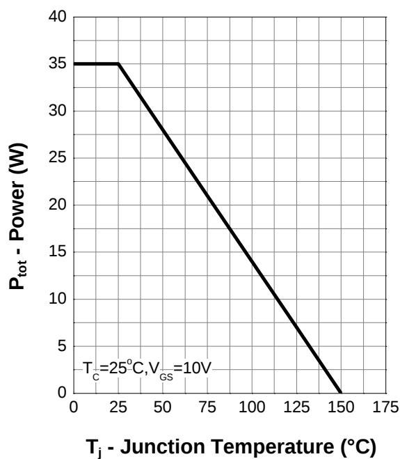
Power Capability
