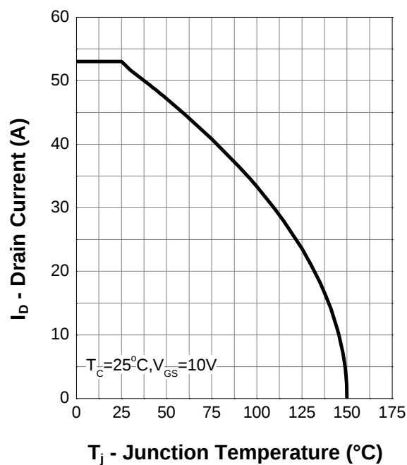
Current Capability
