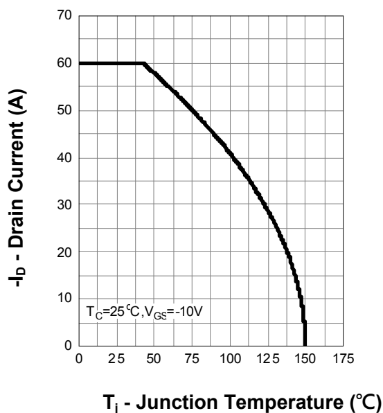
Current Capability
