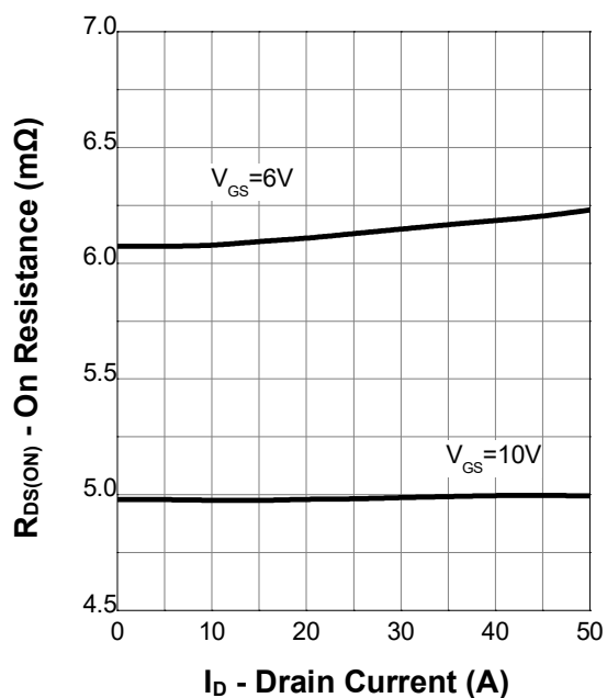
On Resistance
