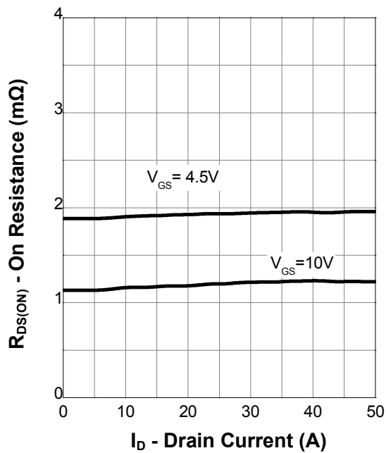
On Resistance
