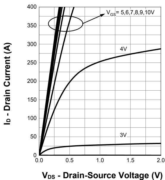
Output Characteristics
