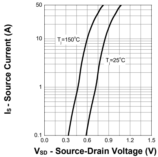
Diode Forward Current
