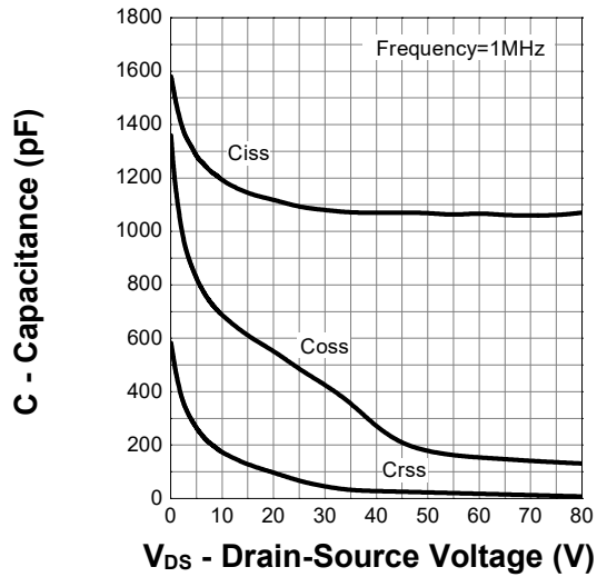
Capacitance
