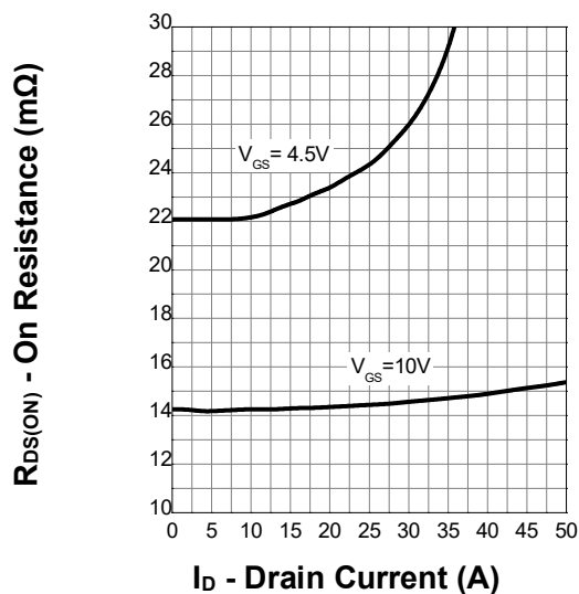
On Resistance
