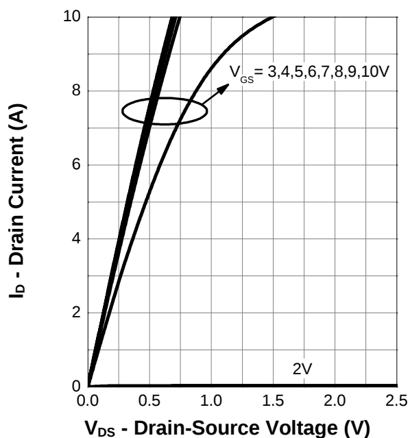
Output Characteristics
