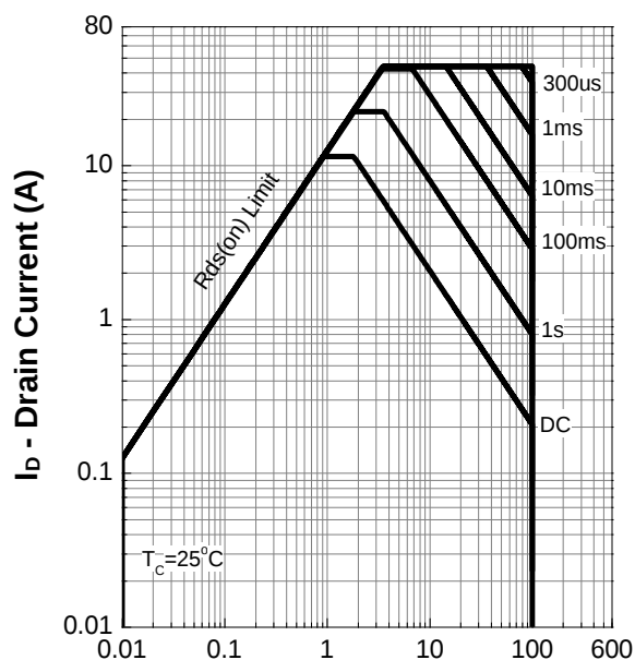
Safe Operation
