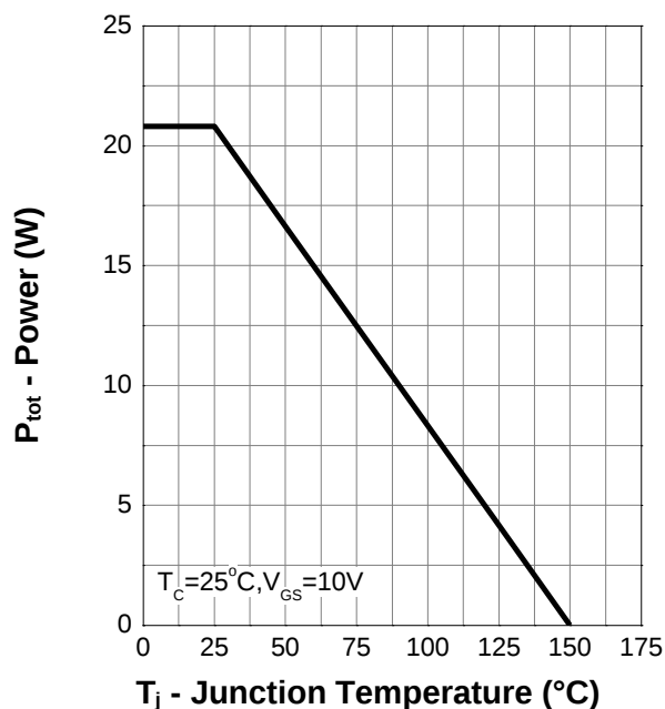
Power Capability
