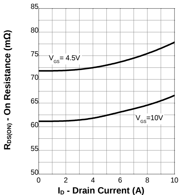
On Resistance
