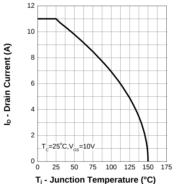
Current Capability
