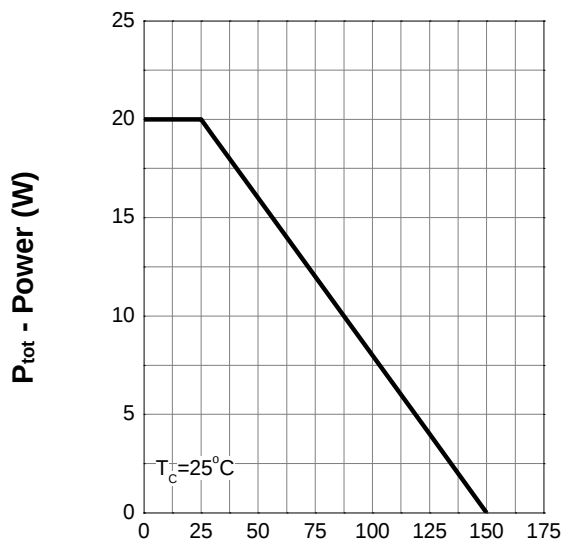
Power Capability
