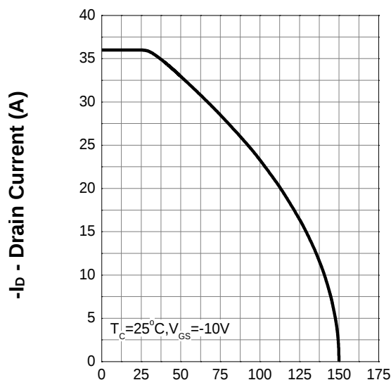
Current Capability
