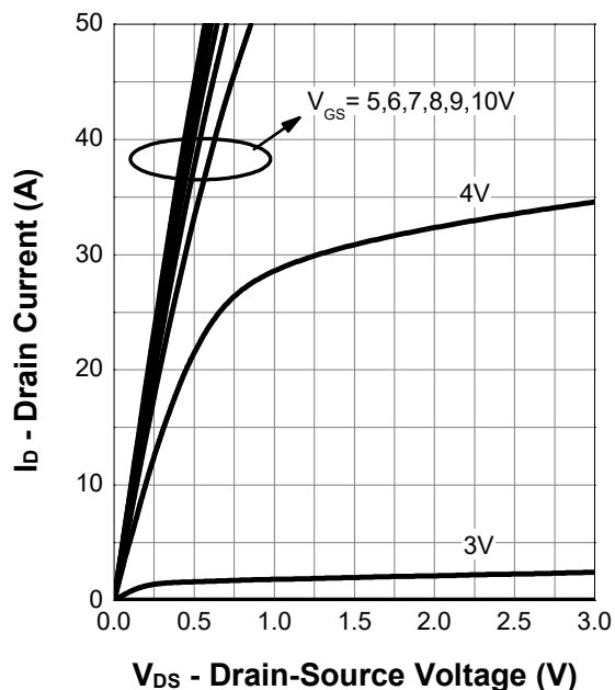
Output Characteristics
