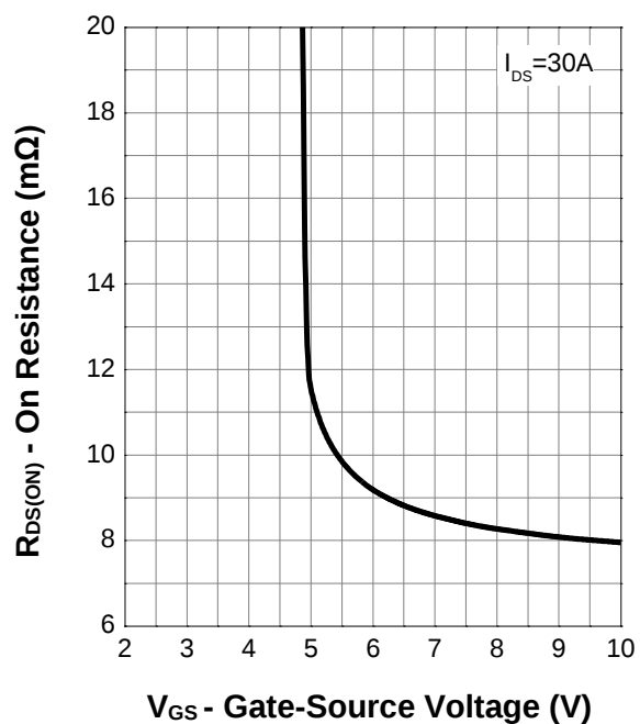
Transfer Characteristics
