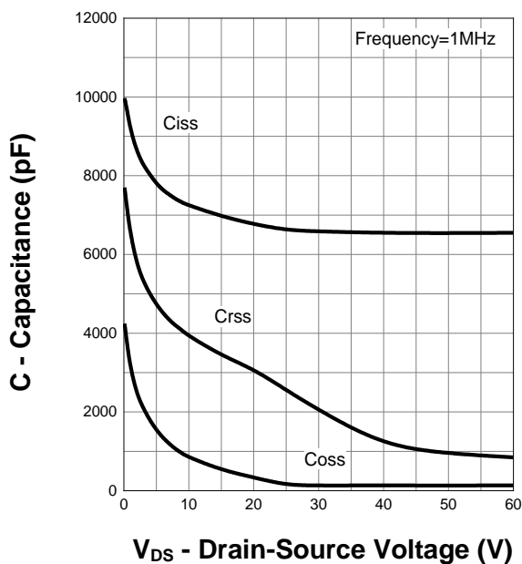
Capacitance
