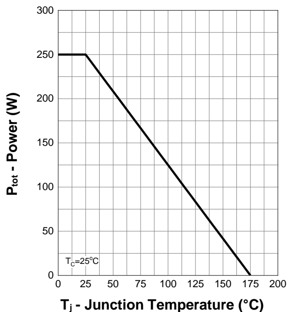
Power Capability
