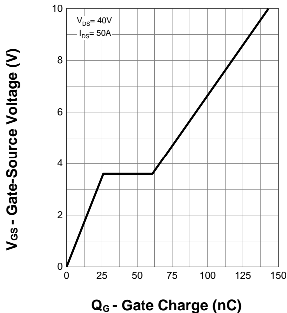
Gate Charge
