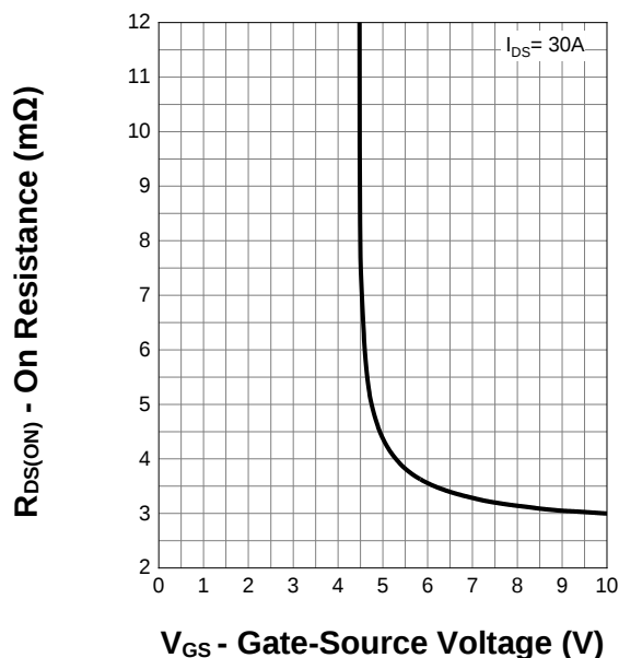
Transfer Characteristics
