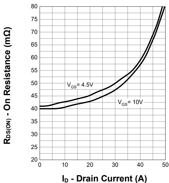
On Resistance
