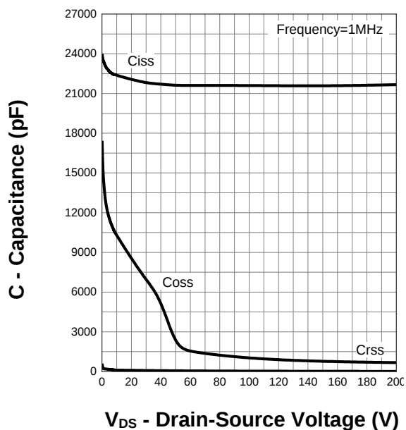
Capacitance
