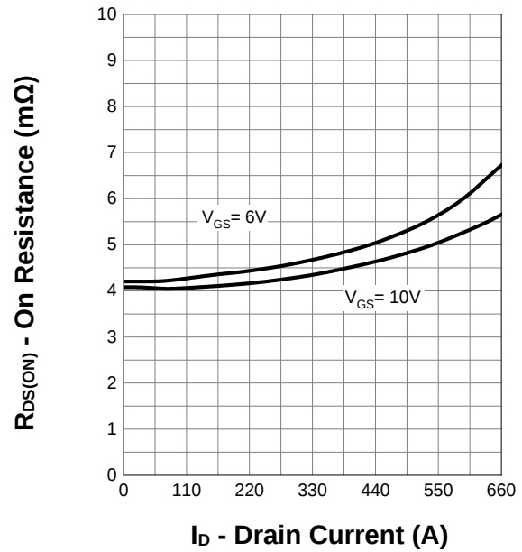
On Resistance
