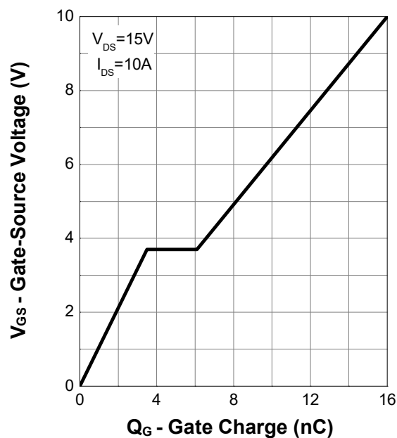
Gate Charge
