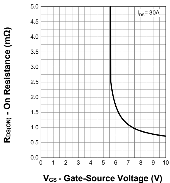
Transfer Characteristics
