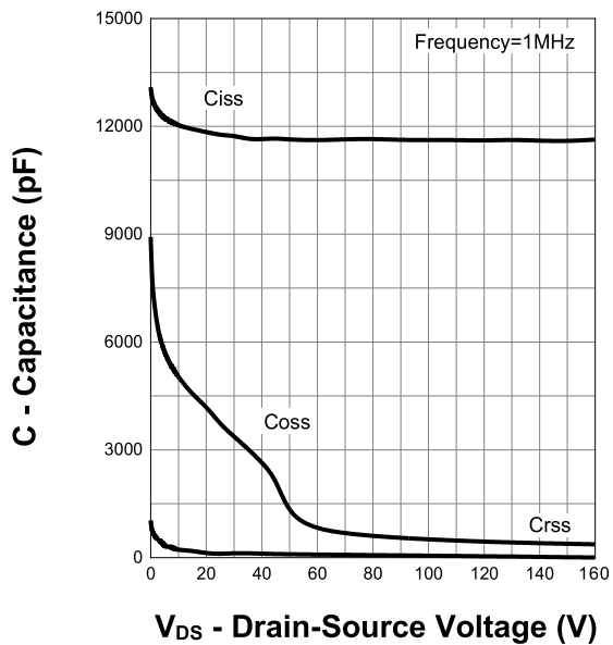
Capacitance
