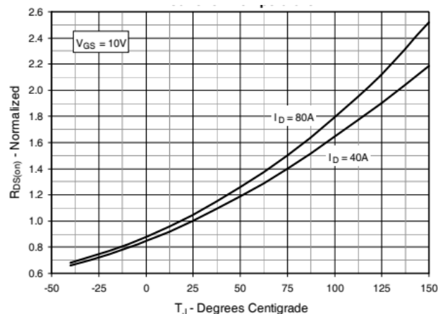
Figure 4. R_{DS(on)} Normalized to I_D=40A Value vs. Junction Temperature
