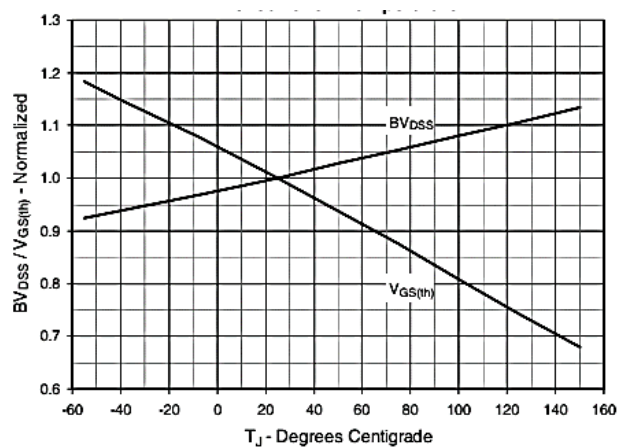
Figure 6. Normalized Breakdown & Threshold Voltages vs. Junction Temperature
