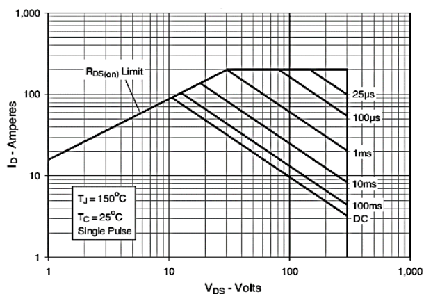
Figure 9. Forward-Bias Safe Operating Area
