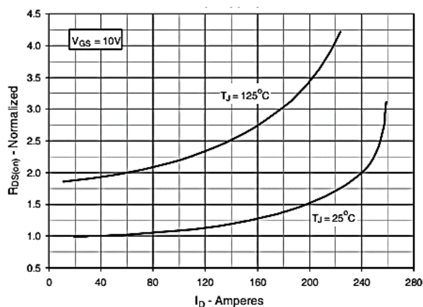
Figure 5. R_{DS(on)} Normalized to I_D=40A Value vs. Drain Current
