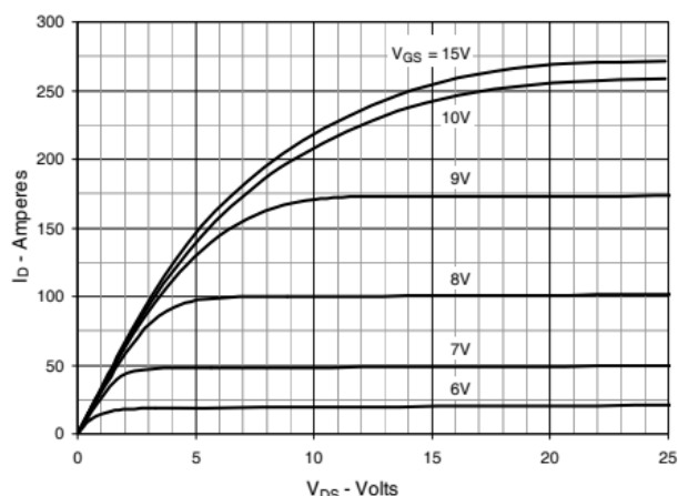
Figure 2. Extended Output Characteristics
