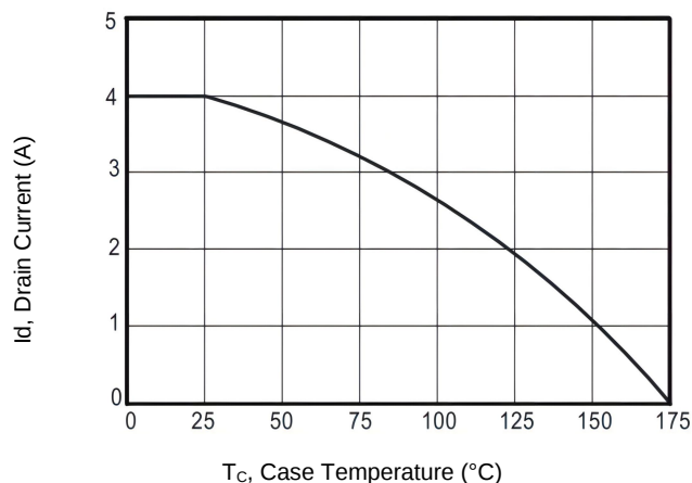
Figure 10. Maximum Continuous Drain Current versus Case Temperature
