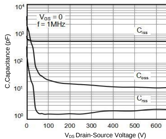
Figure 5. Typical Capacitance versus V_{DS}
