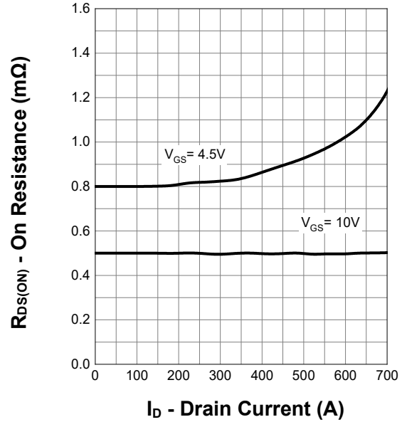
On Resistance
