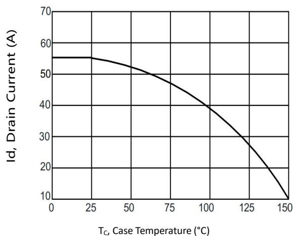
Figure 10. Maximum Continuous Drain versus Case Temperature
