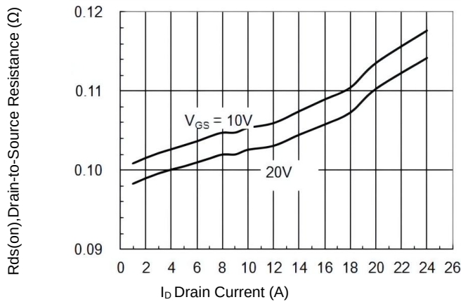
Figure 3. On-Resistance versus Drain Current
