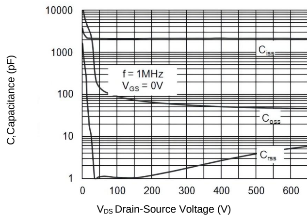
Figure 5. Typical Capacitance versus V_{DS}
